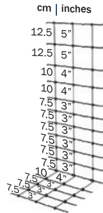
11/90/15 with 32.5cm Hinged Apron
