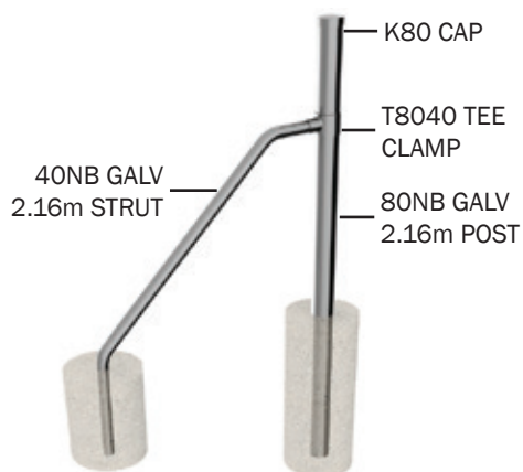
Tubular Strainer 80/40 Heavy Duty
